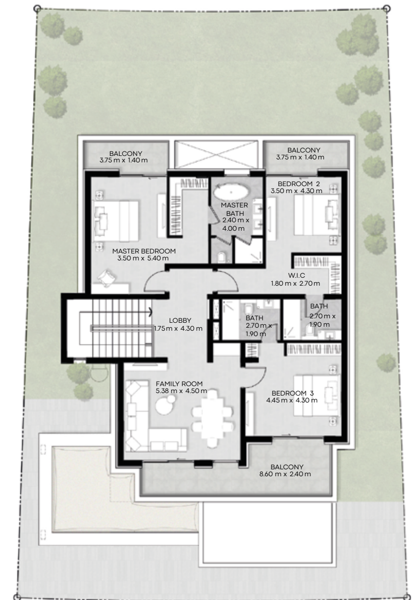
FIRST FLOOR
